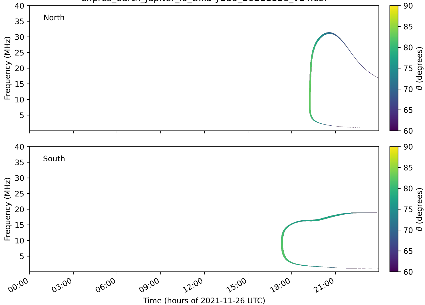
expres_earth_jupiter_io_txka-y235_20211126_v14.cdf
