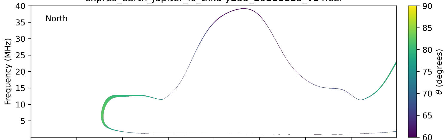
expres_earth_jupiter_io_txka-y235_20211123_v14.cdf
