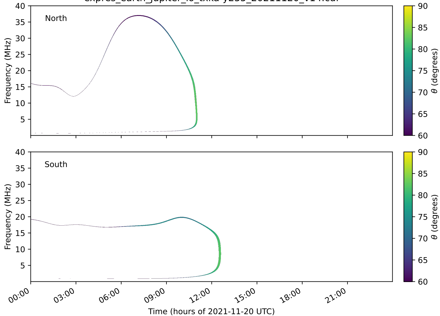
expres_earth_jupiter_io_txka-y235_20211120_v14.cdf
