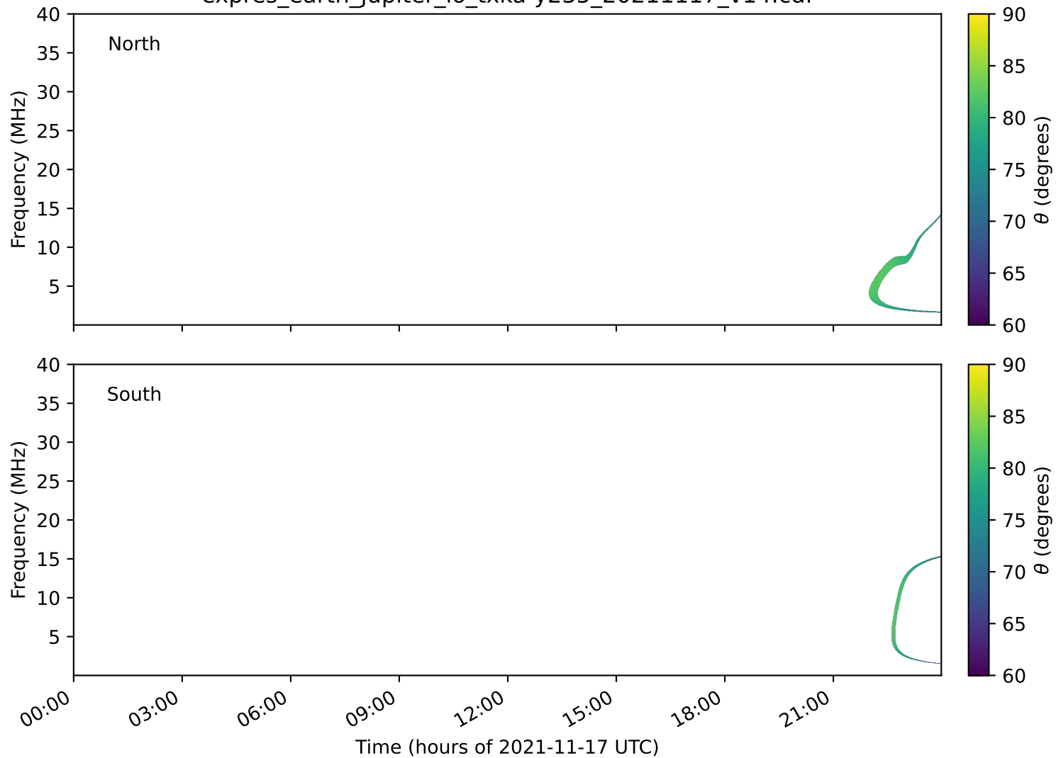
expres_earth_jupiter_io_txka-y235_20211117_v14.cdf
