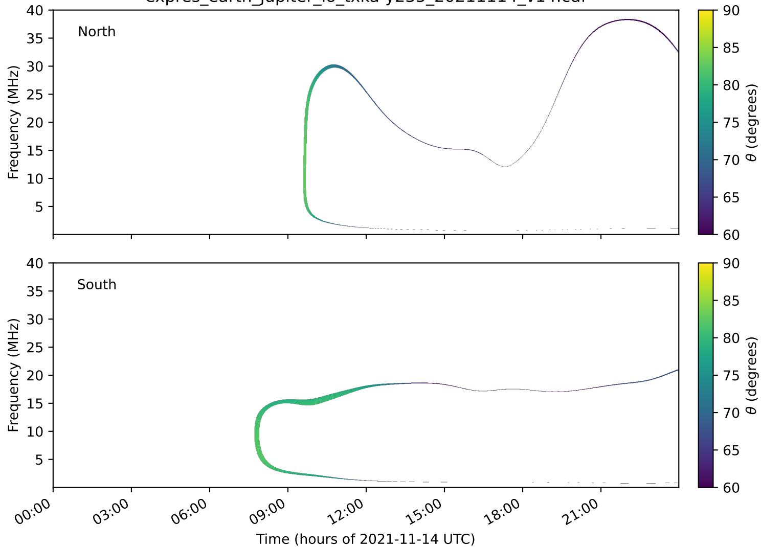
expres_earth_jupiter_io_txka-y235_20211114_v14.cdf
