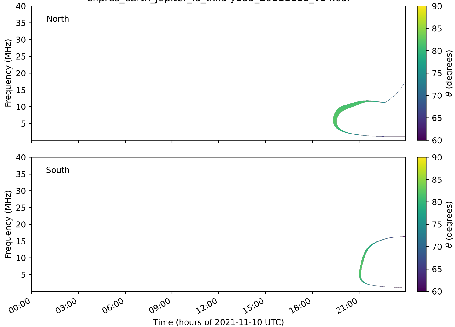
expres_earth_jupiter_io_txka-y235_20211110_v14.cdf
