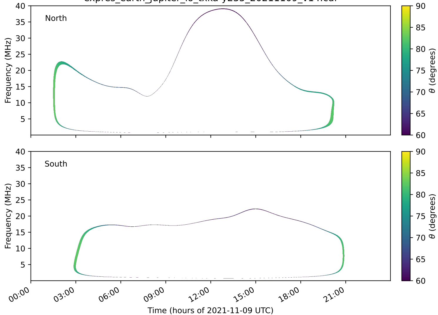
expres_earth_jupiter_io_txka-y235_20211109_v14.cdf
