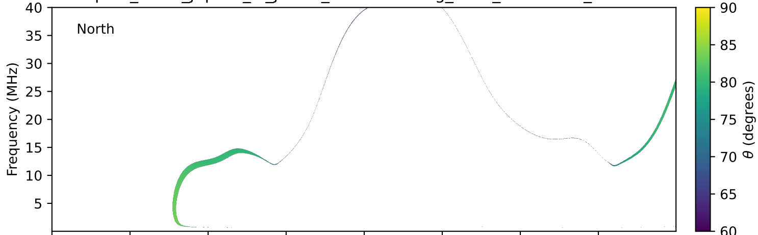
expres_earth_jupiter_io_jrm33_lossc-wid1deg_3kev_20211123_v11.cdf
