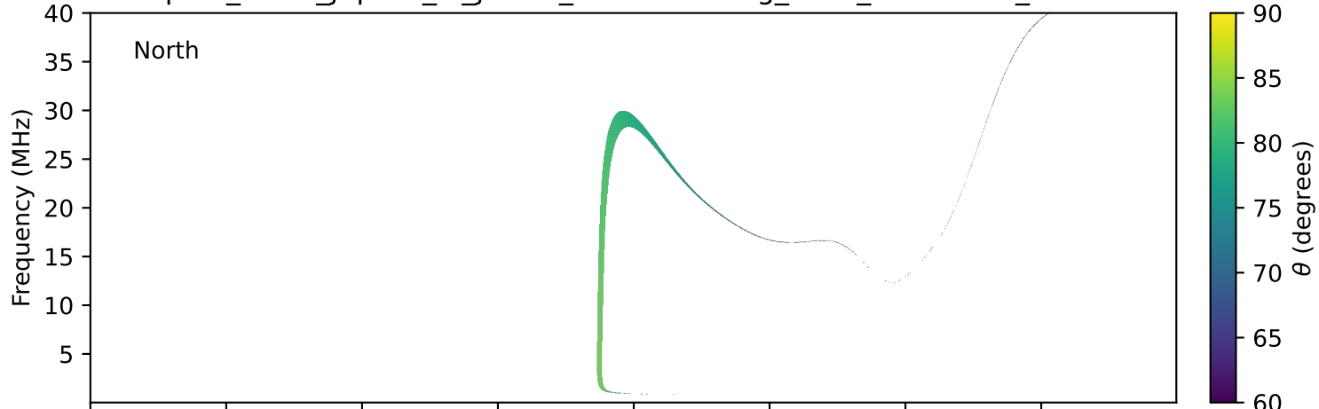
expres_earth_jupiter_io_jrm33_lossc-wid1deg_3kev_20211121_v11.cdf
