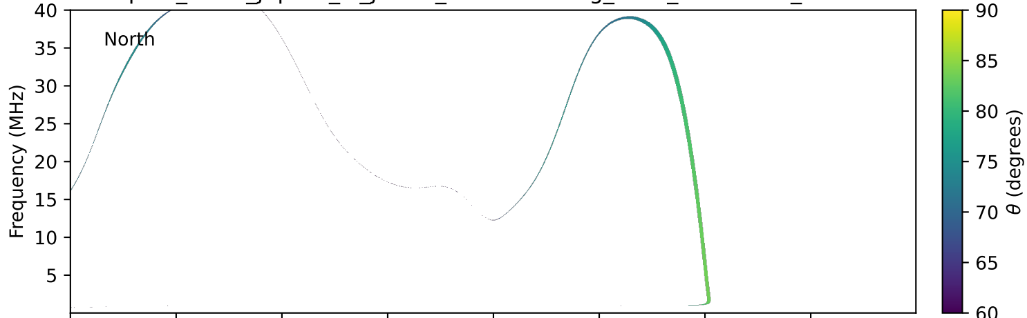
expres_earth_jupiter_io_jrm33_lossc-wid1deg_3kev_20211118_v11.cdf
