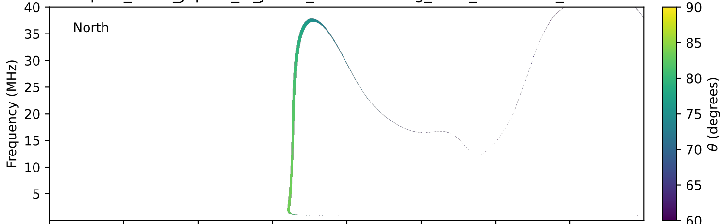
expres_earth_jupiter_io_jrm33_lossc-wid1deg_3kev_20211114_v11.cdf
