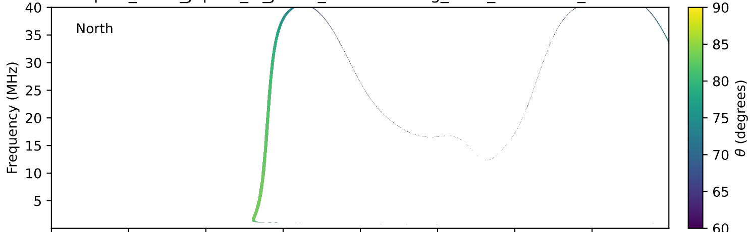
expres_earth_jupiter_io_jrm33_lossc-wid1deg_3kev_20211107_v11.cdf
