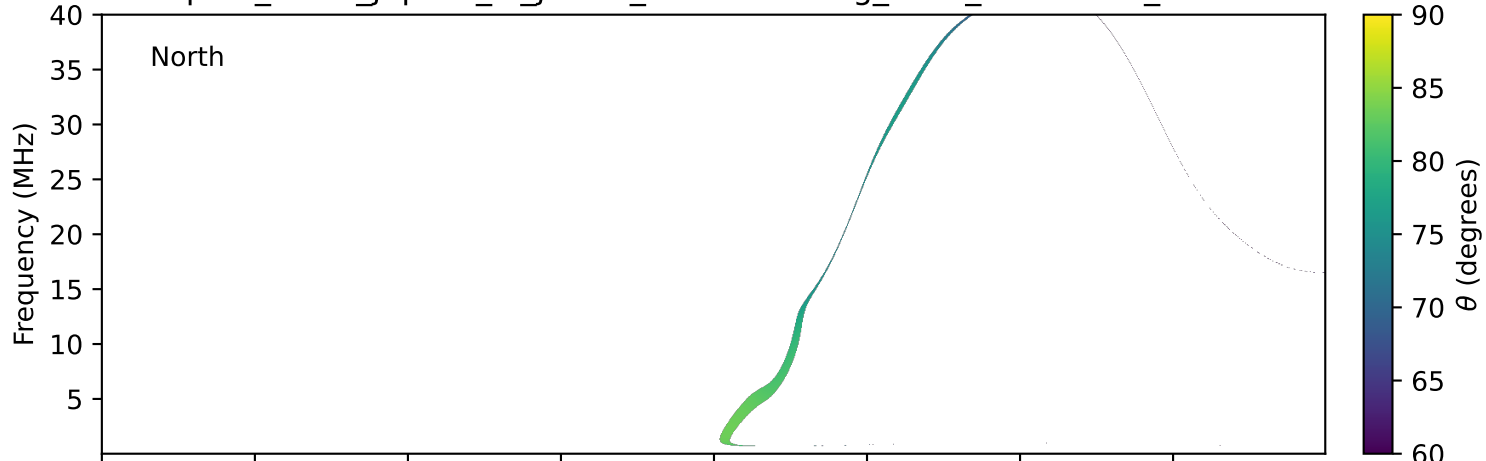
expres_earth_jupiter_io_jrm33_lossc-wid1deg_3kev_20211105_v11.cdf
