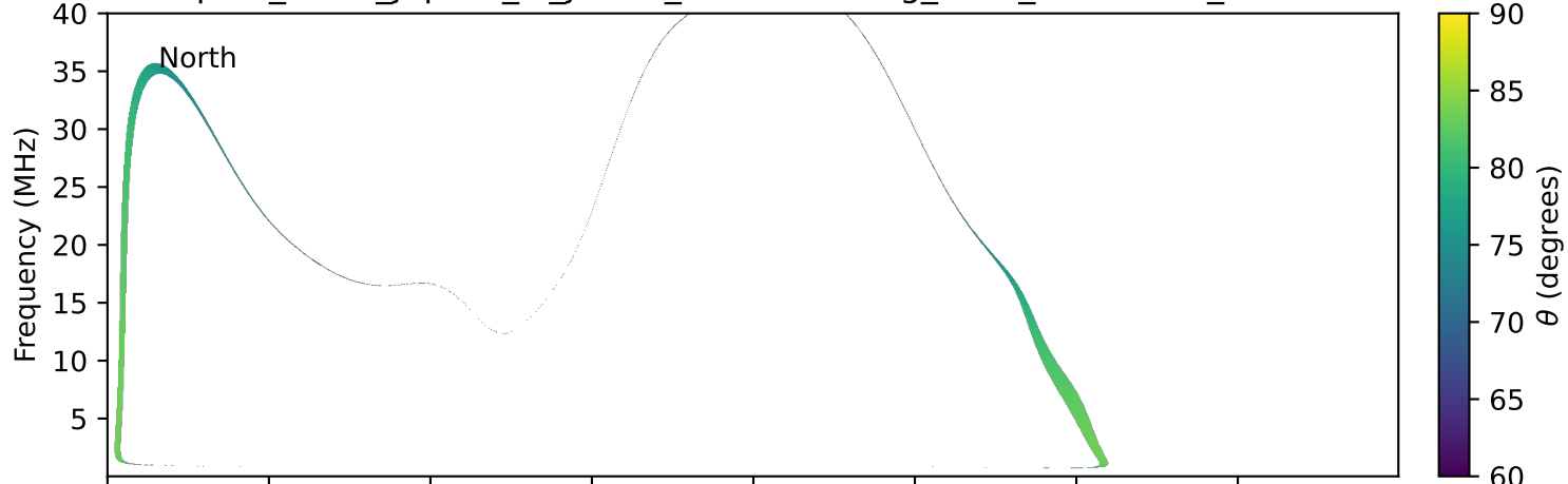
expres_earth_jupiter_io_jrm33_lossc-wid1deg_3kev_20211102_v11.cdf
