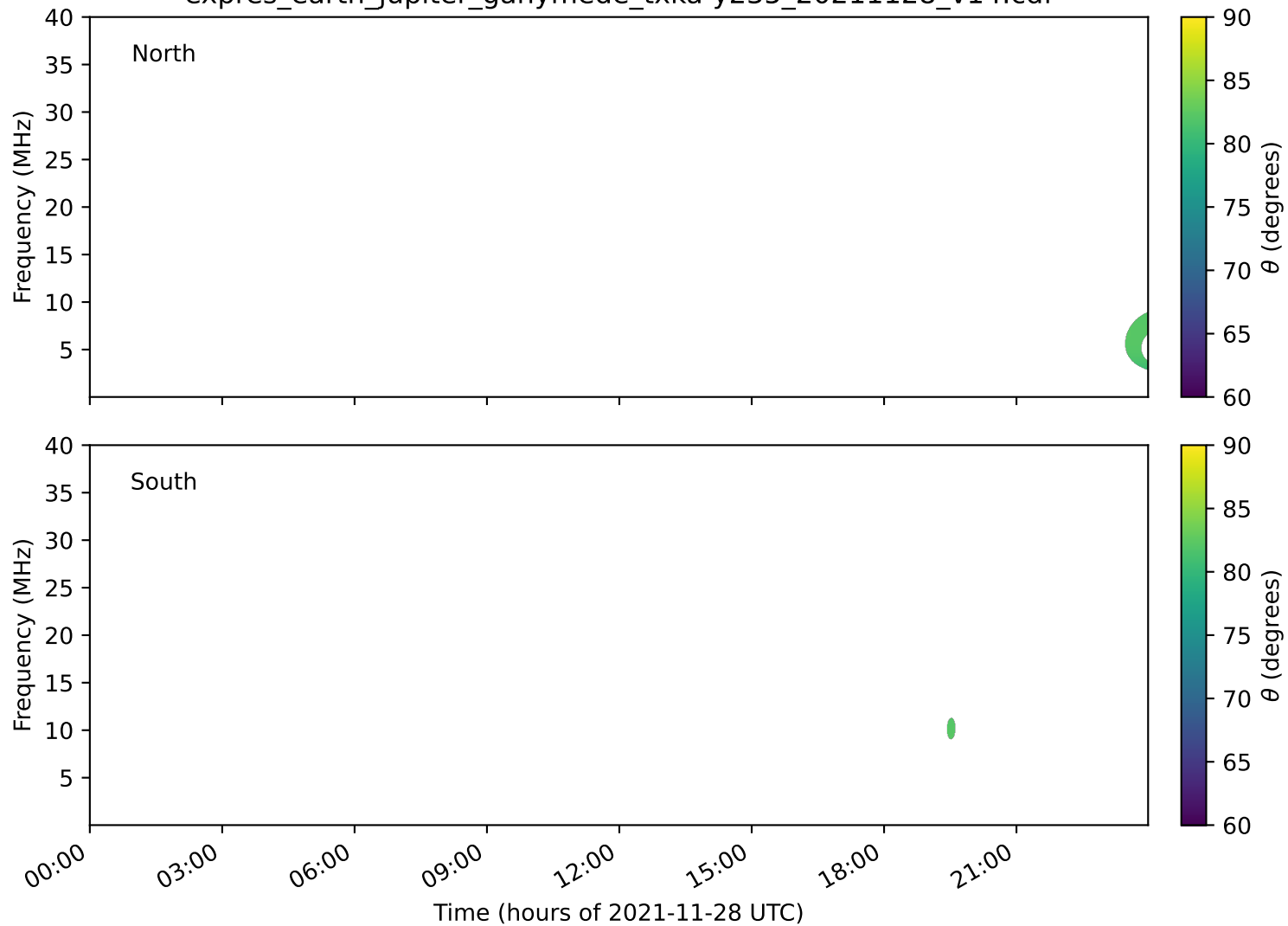
expres_earth_jupiter_ganymede_txka-y235_20211128_v14.cdf
