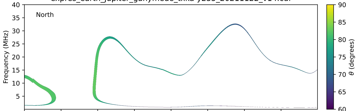
expres_earth_jupiter_ganymede_txka-y235_20211122_v14.cdf
