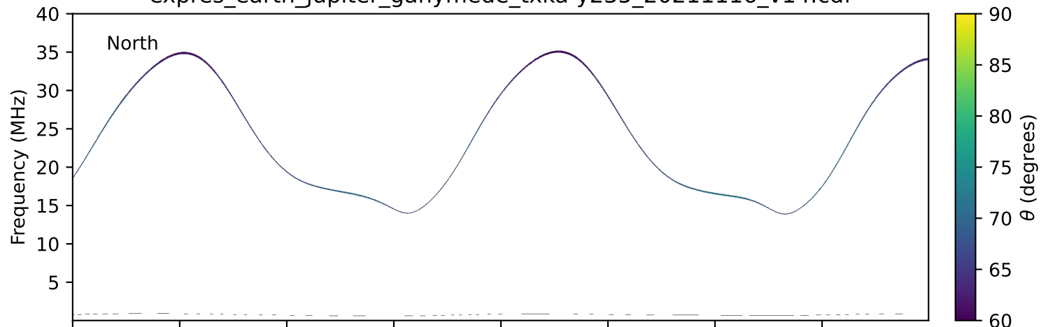
expres_earth_jupiter_ganymede_txka-y235_20211116_v14.cdf
