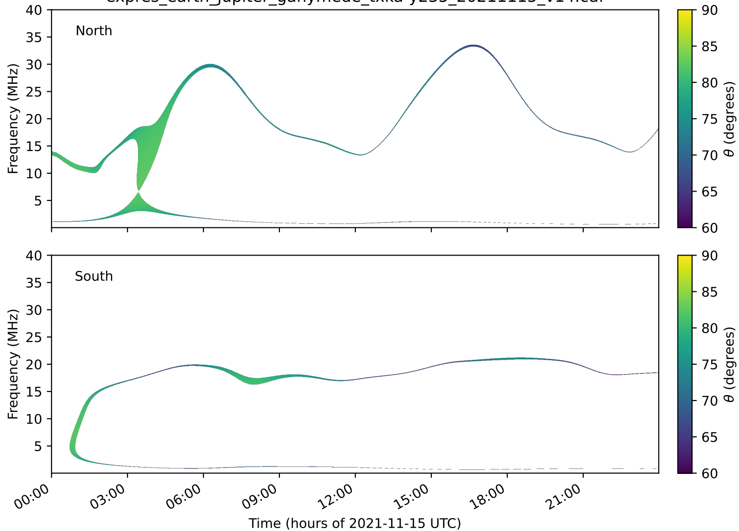
expres_earth_jupiter_ganymede_txka-y235_20211115_v14.cdf
