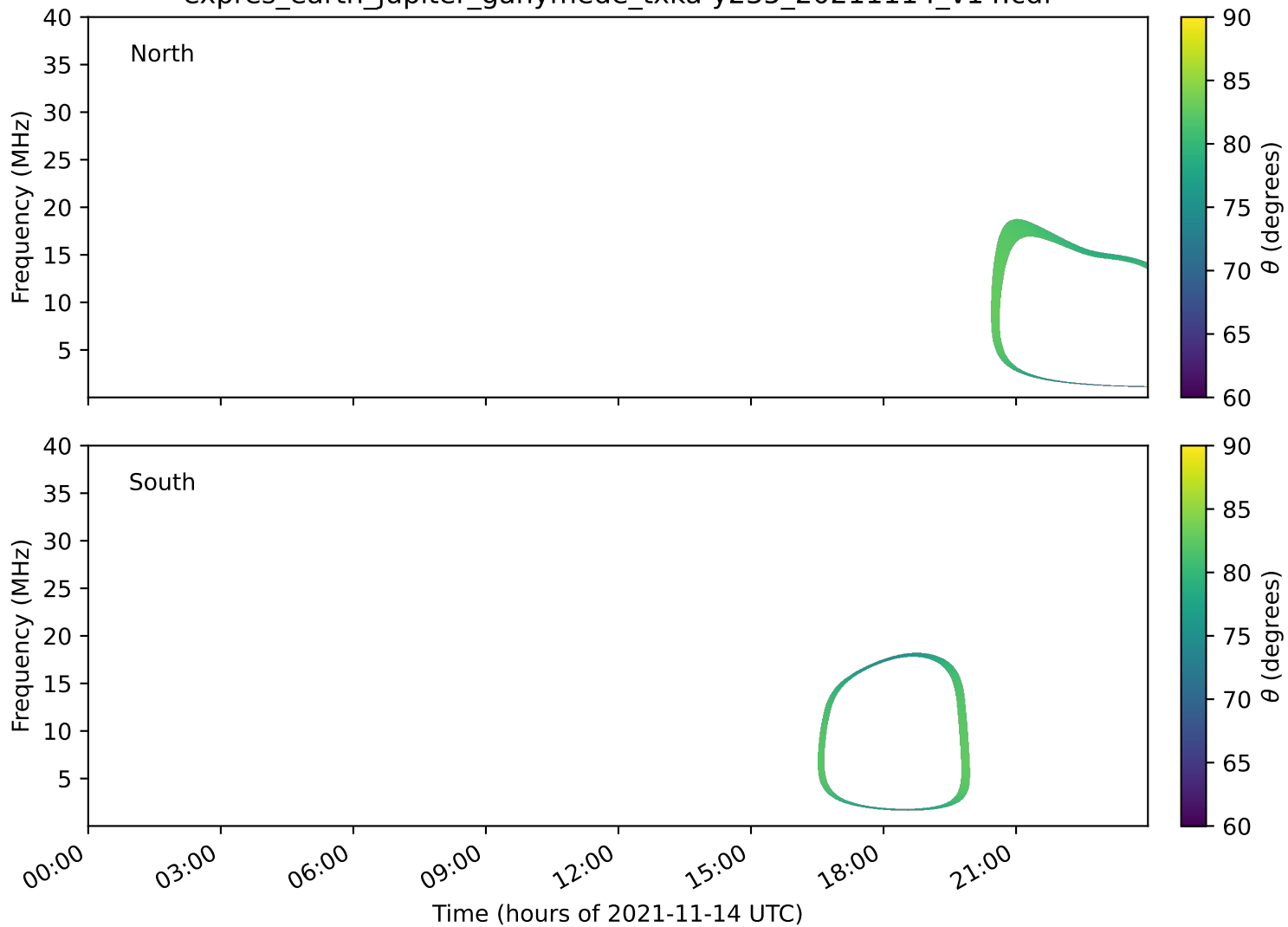
expres_earth_jupiter_ganymede_txka-y235_20211114_v14.cdf
