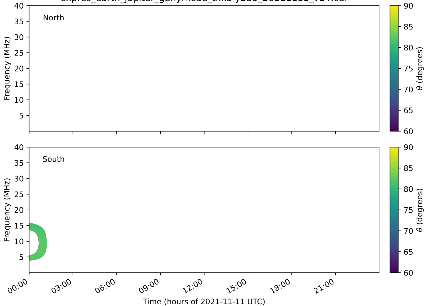
expres_earth_jupiter_ganymede_txka-y235_20211111_v14.cdf
