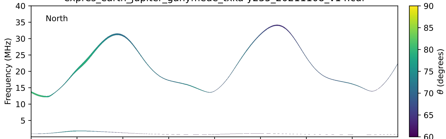
expres_earth_jupiter_ganymede_txka-y235_20211108_v14.cdf
