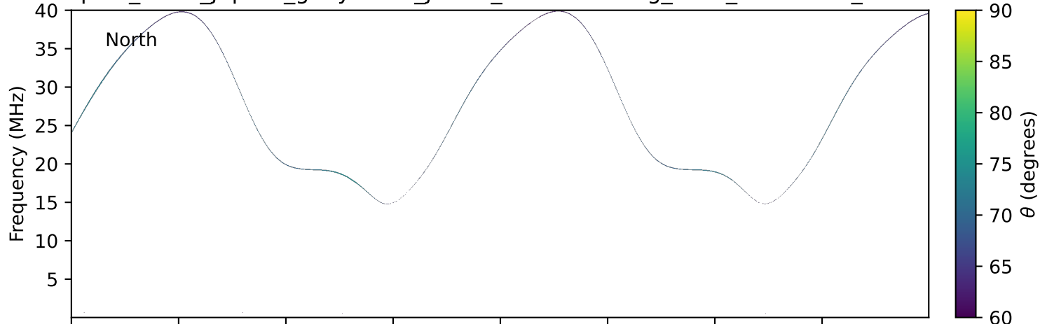
expres_earth_jupiter_ganymede_jrm33_lossc-wid1deg_3kev_20211116_v11.cdf
