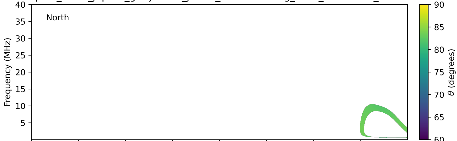
expres_earth_jupiter_ganymede_jrm33_lossc-wid1deg_3kev_20211114_v11.cdf
