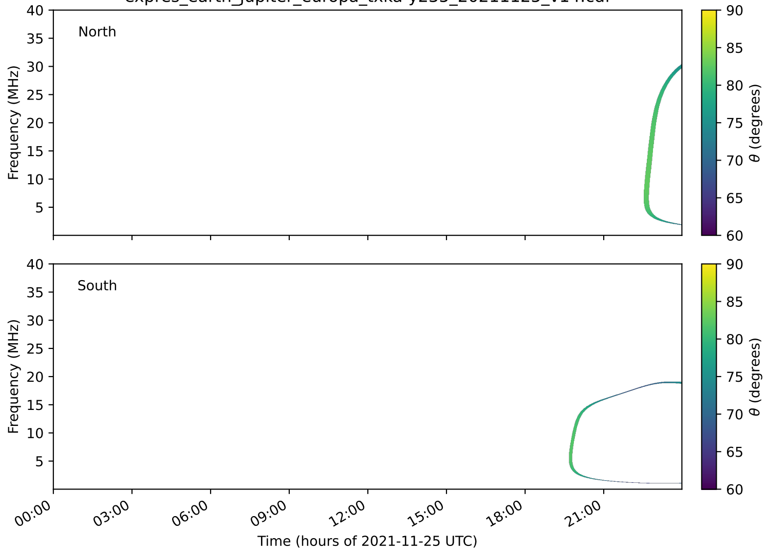
expres_earth_jupiter_europa_txka-y235_20211125_v14.cdf
