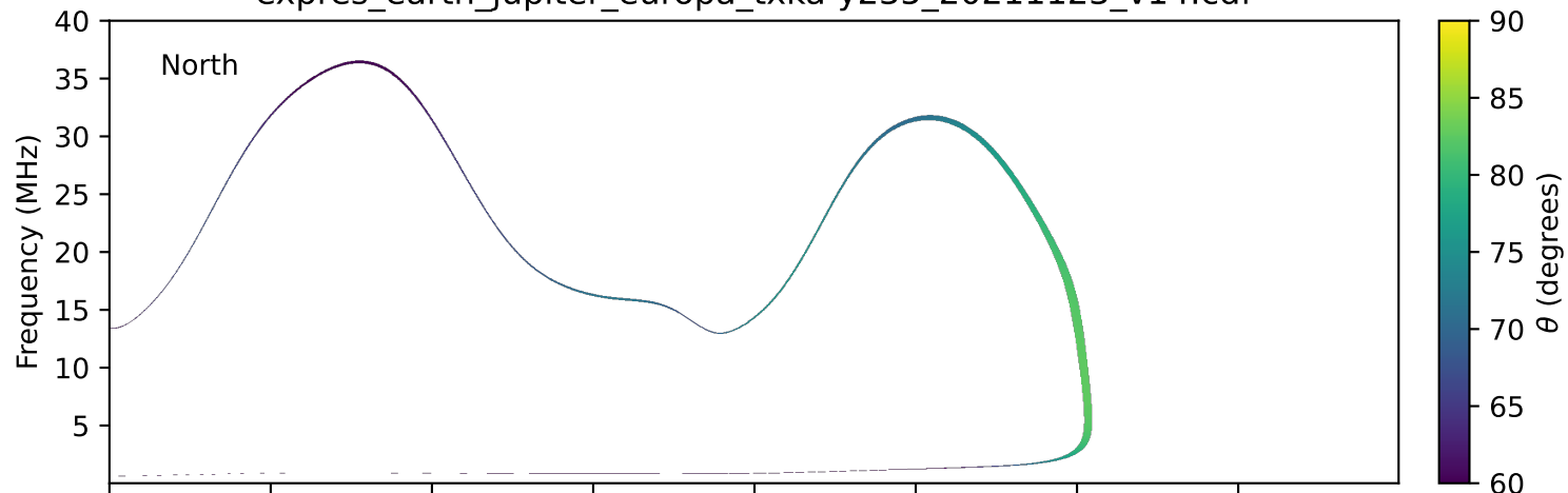
expres_earth_jupiter_europa_txka-y235_20211123_v14.cdf
