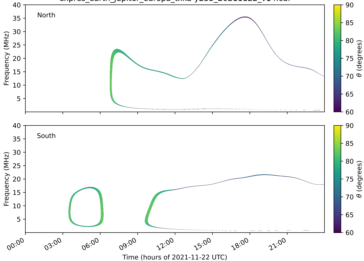
expres_earth_jupiter_europa_txka-y235_20211122_v14.cdf
