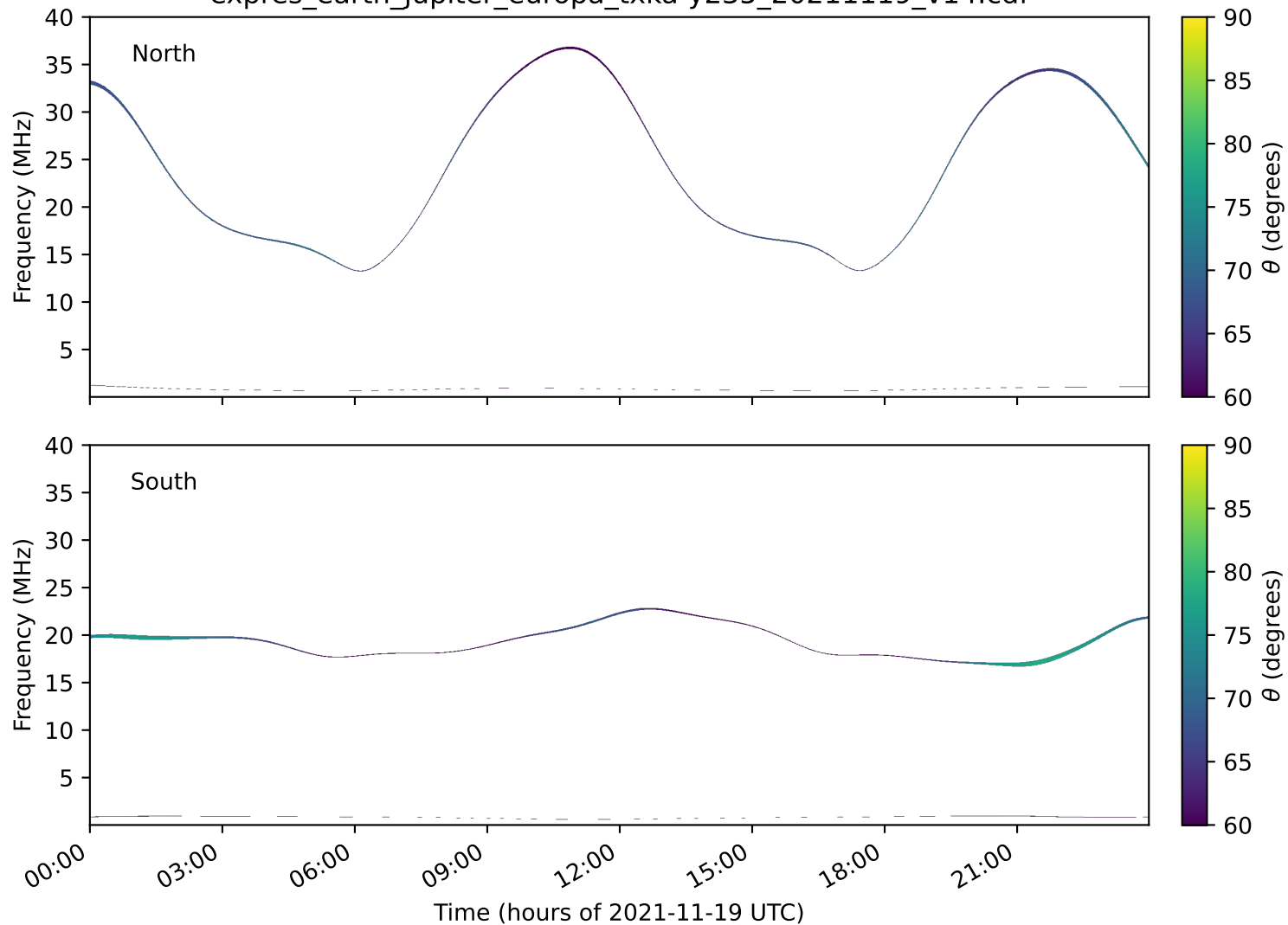
expres_earth_jupiter_europa_txka-y235_20211119_v14.cdf
