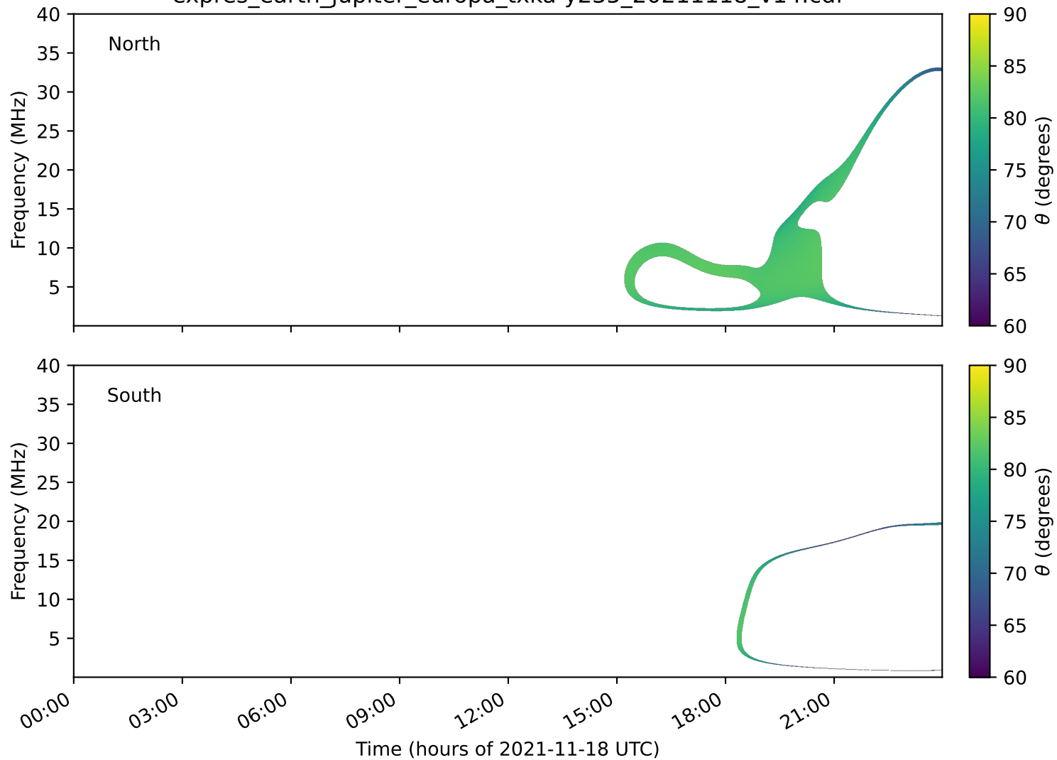
expres_earth_jupiter_europa_txka-y235_20211118_v14.cdf
