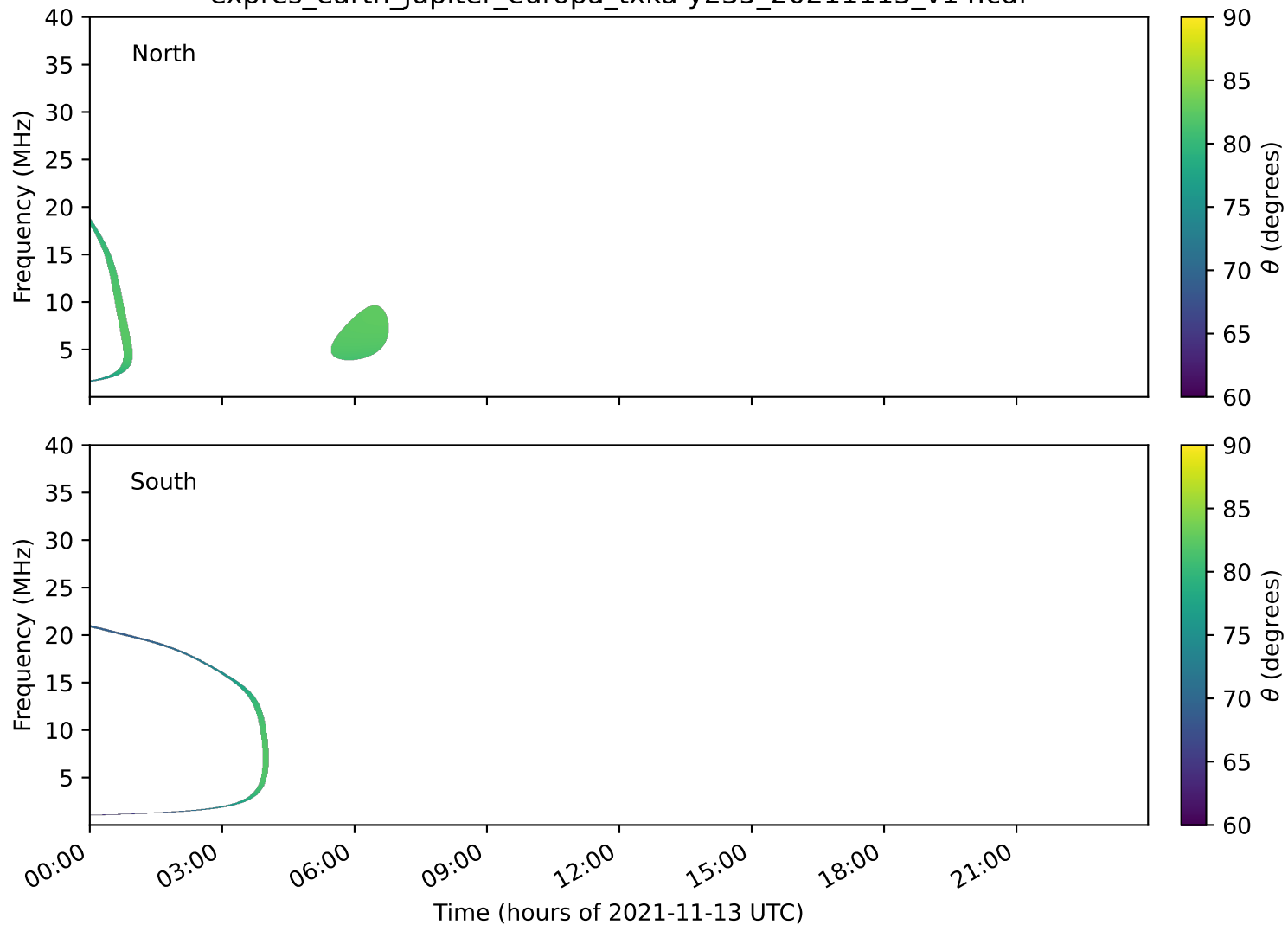
expres_earth_jupiter_europa_txka-y235_20211113_v14.cdf
