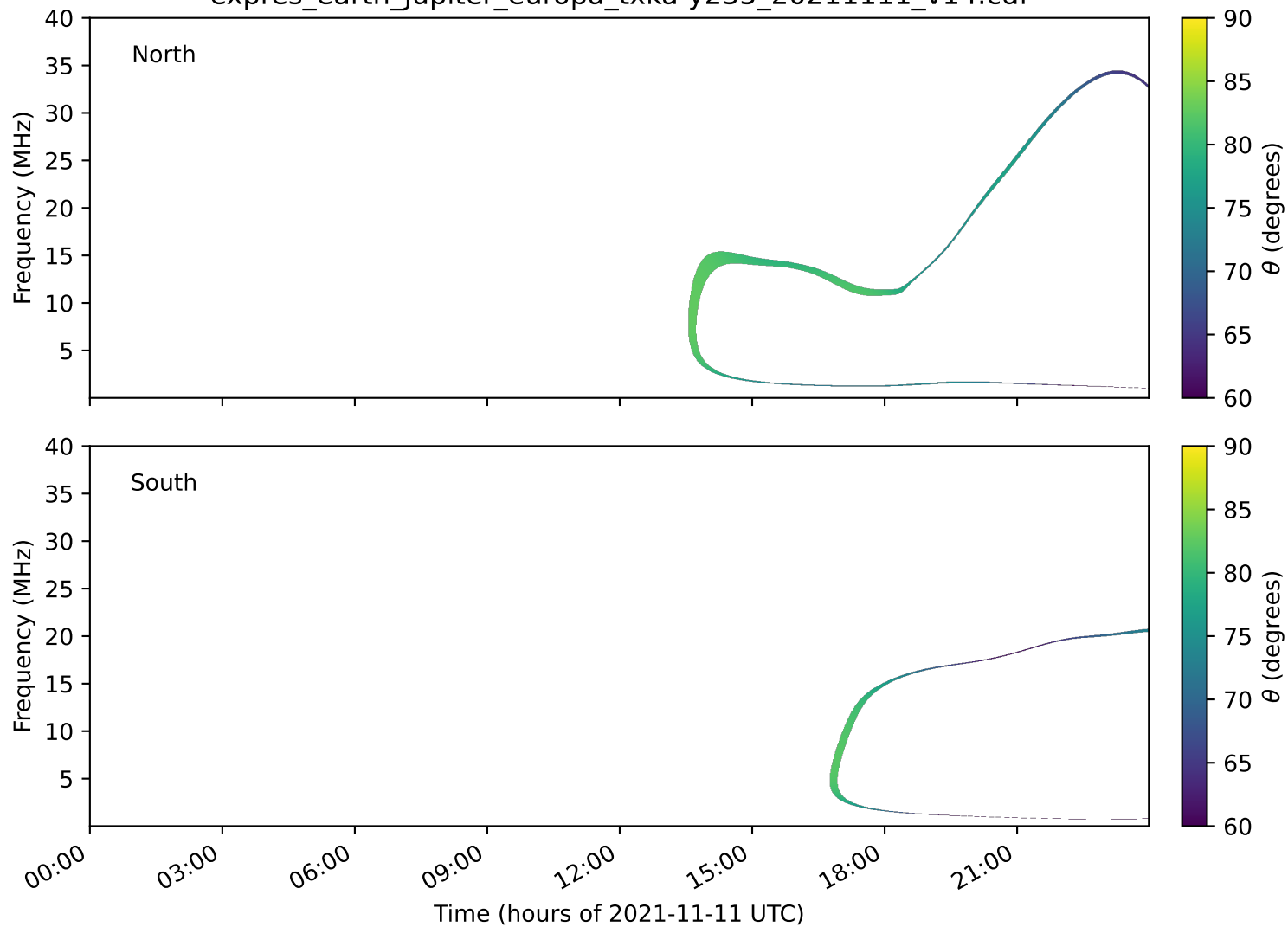
expres_earth_jupiter_europa_txka-y235_20211111_v14.cdf
