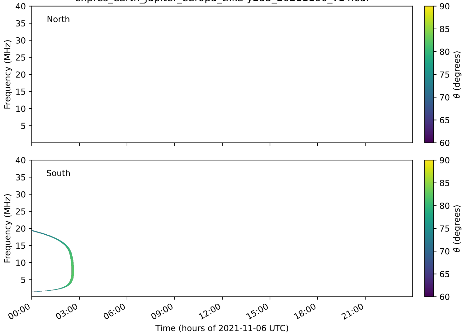
expres_earth_jupiter_europa_txka-y235_20211106_v14.cdf
