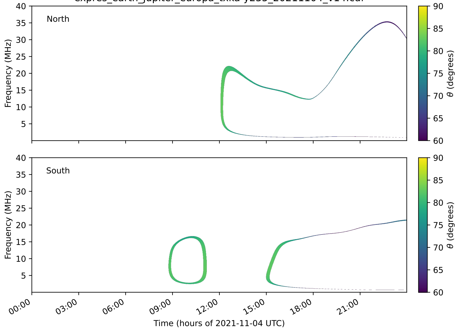
expres_earth_jupiter_europa_txka-y235_20211104_v14.cdf
