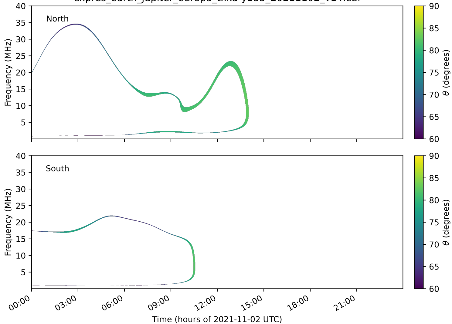
expres_earth_jupiter_europa_txka-y235_20211102_v14.cdf
