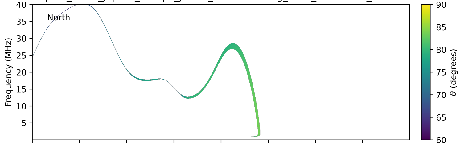
expres_earth_jupiter_europa_jrm33_lossc-wid1deg_3kev_20211102_v11.cdf
