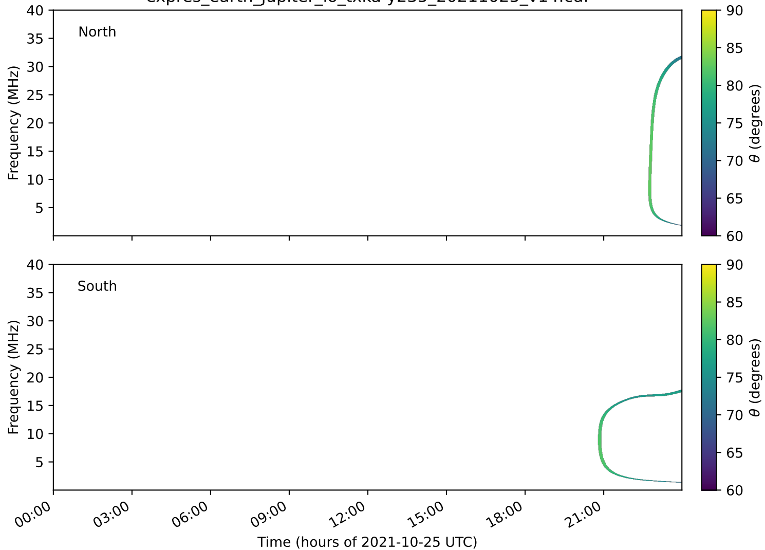
expres_earth_jupiter_io_txka-y235_20211025_v14.cdf
