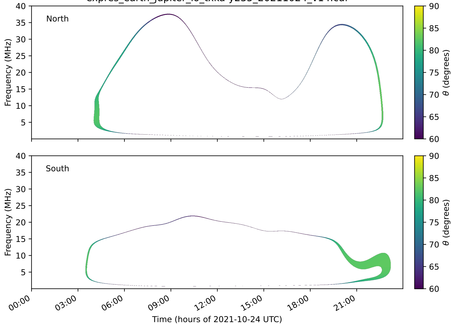
expres_earth_jupiter_io_txka-y235_20211024_v14.cdf
