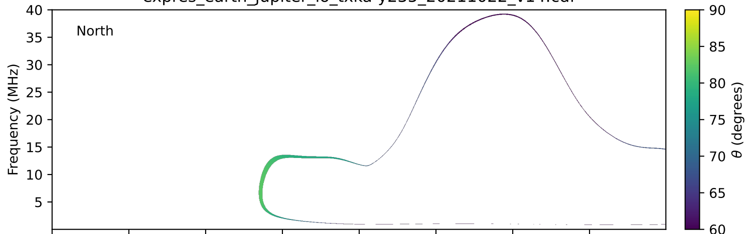
expres_earth_jupiter_io_txka-y235_20211022_v14.cdf
