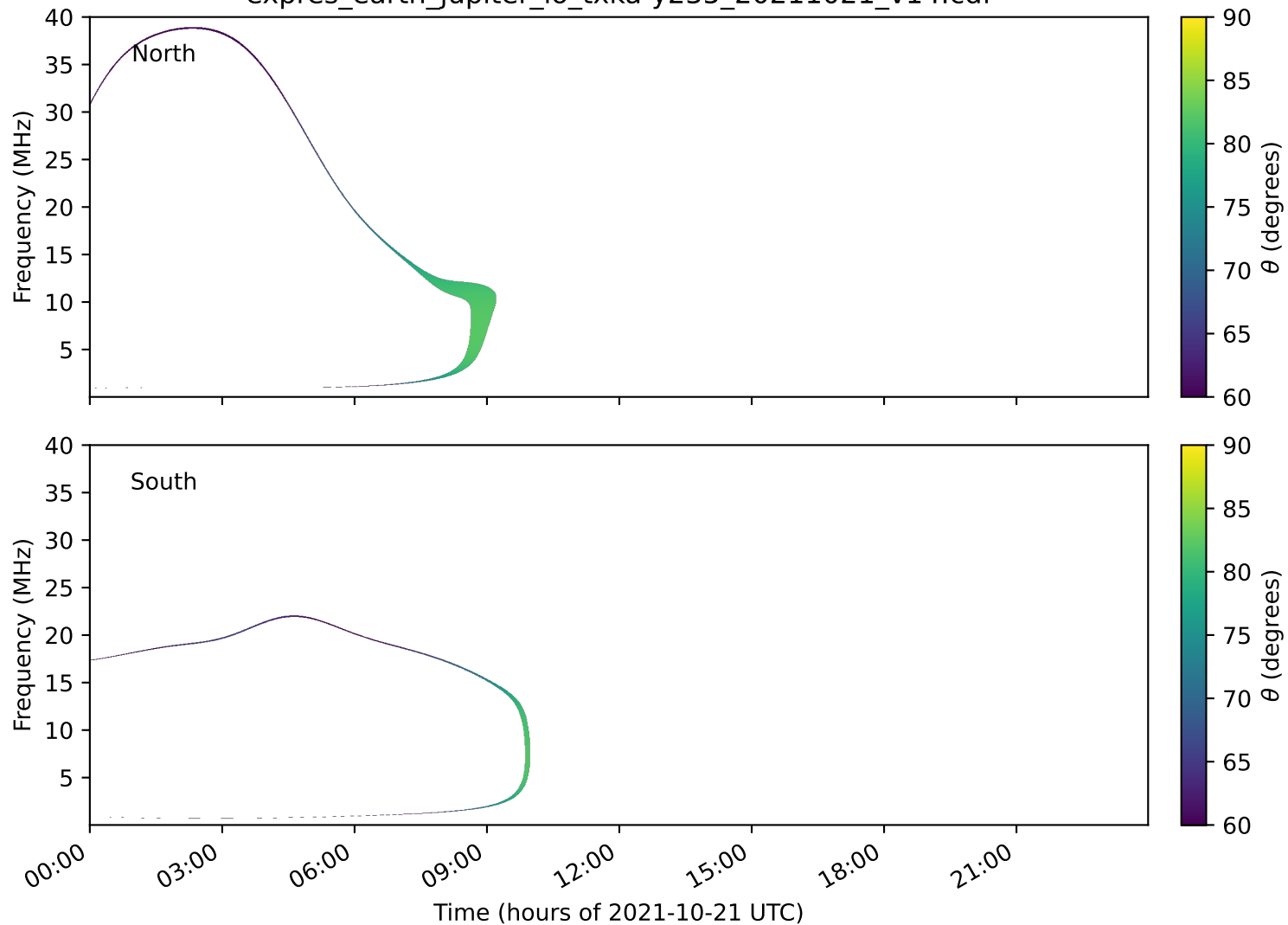
expres_earth_jupiter_io_txka-y235_20211021_v14.cdf
