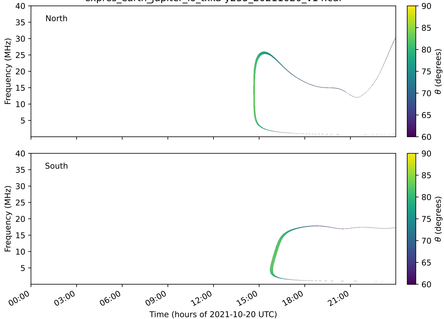
expres_earth_jupiter_io_txka-y235_20211020_v14.cdf
