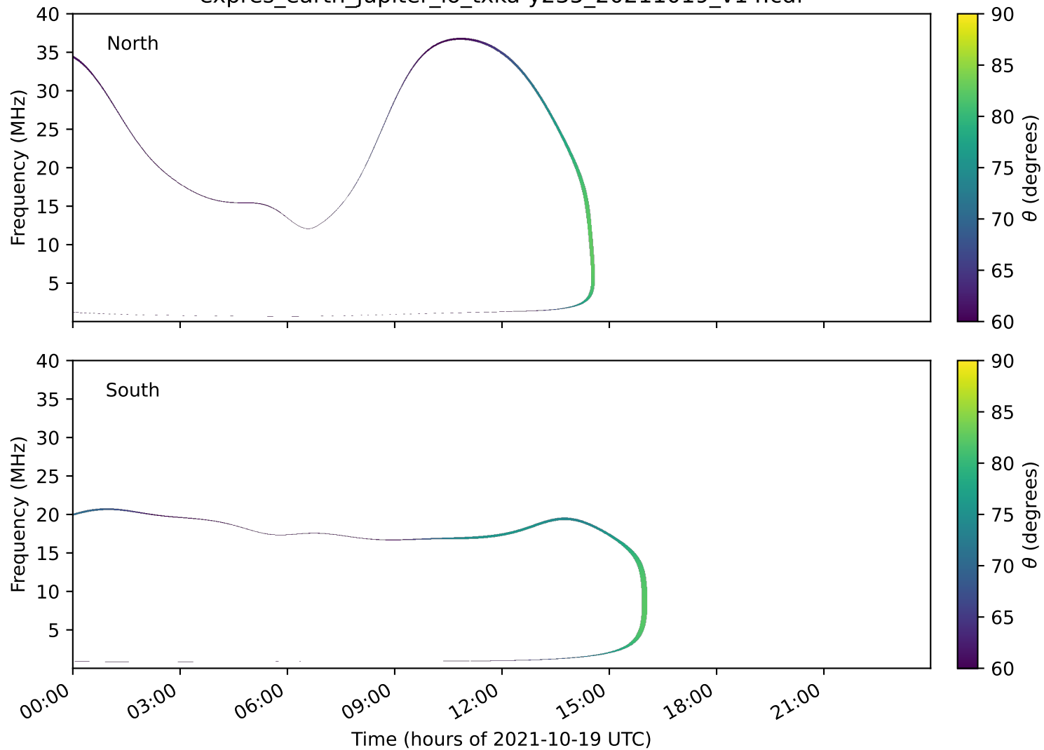
expres_earth_jupiter_io_txka-y235_20211019_v14.cdf
