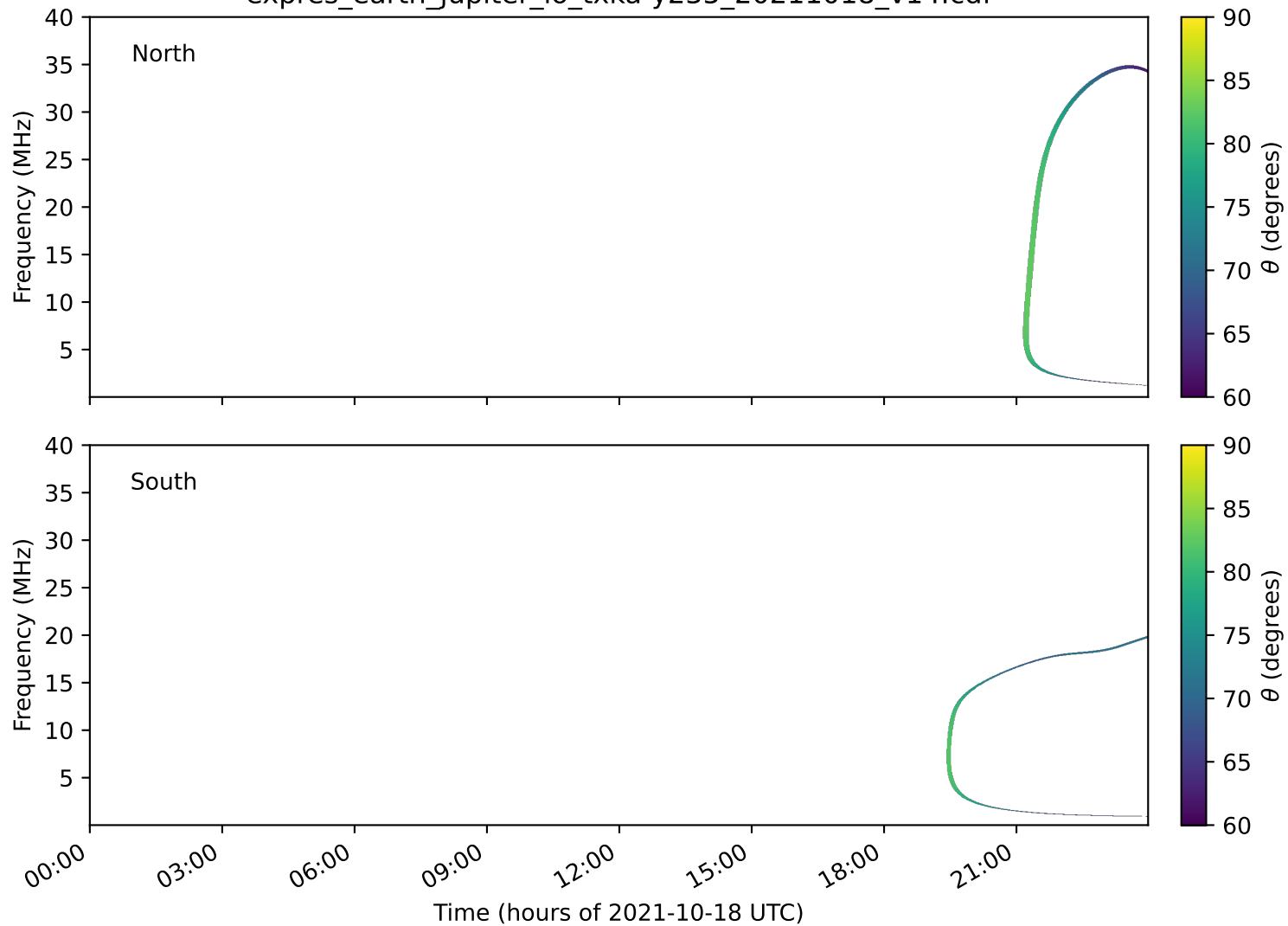
expres_earth_jupiter_io_txka-y235_20211018_v14.cdf
