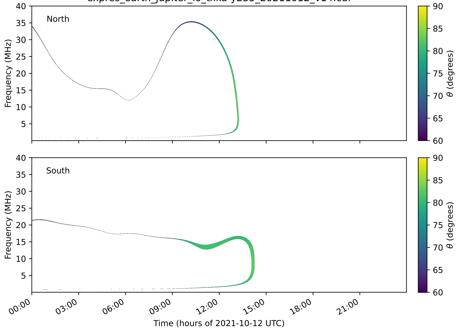
expres_earth_jupiter_io_txka-y235_20211012_v14.cdf
