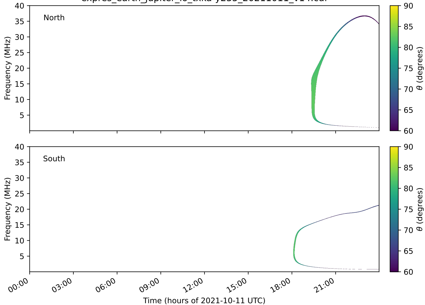
expres_earth_jupiter_io_txka-y235_20211011_v14.cdf
