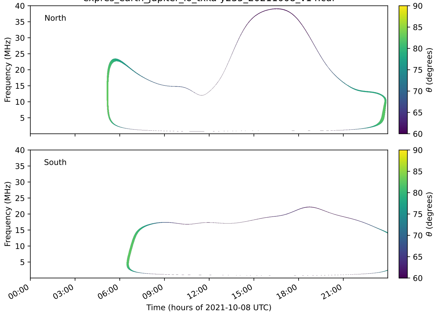
expres_earth_jupiter_io_txka-y235_20211008_v14.cdf
