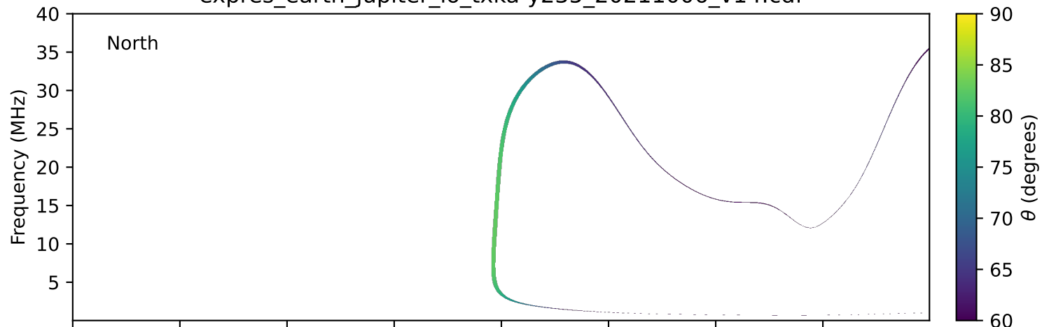
expres_earth_jupiter_io_txka-y235_20211006_v14.cdf
