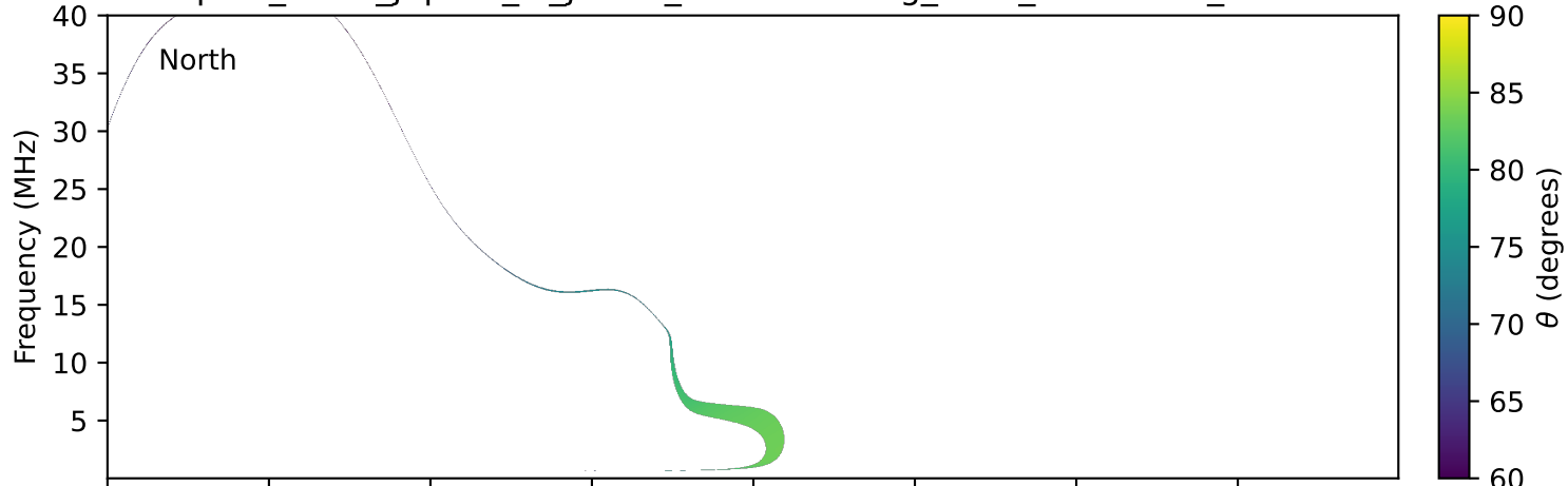
expres_earth_jupiter_io_jrm33_lossc-wid1deg_3kev_20211028_v11.cdf
