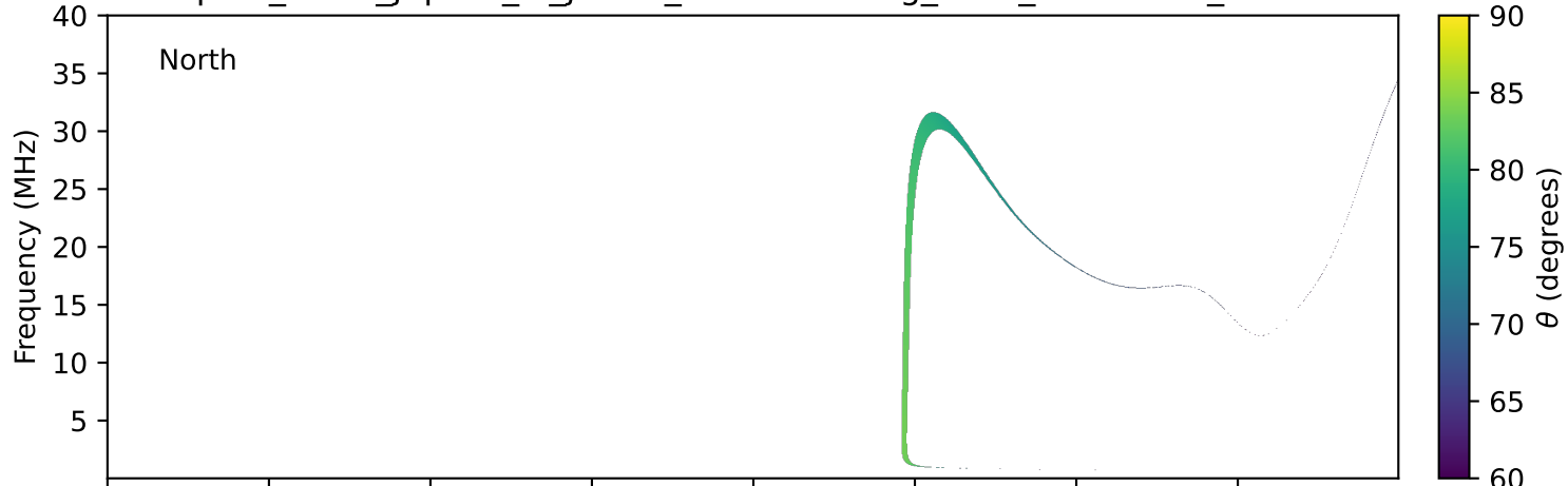
expres_earth_jupiter_io_jrm33_lossc-wid1deg_3kev_20211020_v11.cdf
