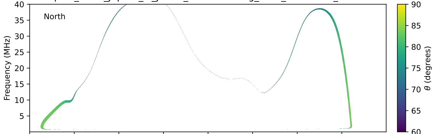
expres_earth_jupiter_io_jrm33_lossc-wid1deg_3kev_20211017_v11.cdf
