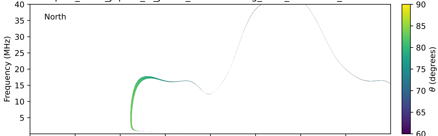
expres_earth_jupiter_io_jrm33_lossc-wid1deg_3kev_20211015_v11.cdf
