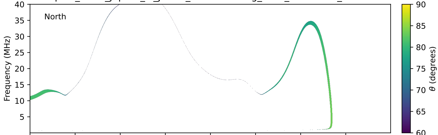
expres_earth_jupiter_io_jrm33_lossc-wid1deg_3kev_20211010_v11.cdf
